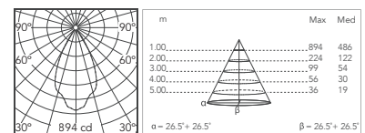
Preliminary photometry
