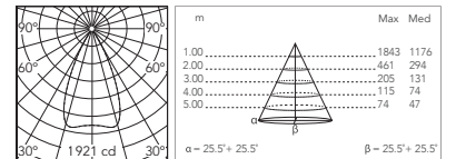
Preliminary photometry
