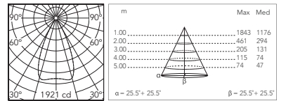
Preliminary photometry
