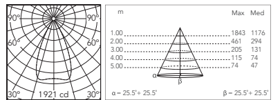
Preliminary photometry
