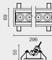
POWER LED 2,7W x SPOT
