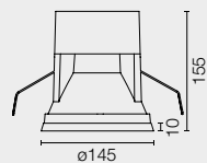
LED ARRAY 36W
