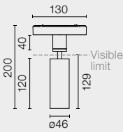
ANTHONY SPOT TRACK
